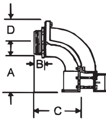
Sizes 2 - 4"
